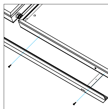
Figure 8. Collector mounting
