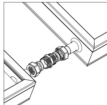
Figure 7. Collector connectors
