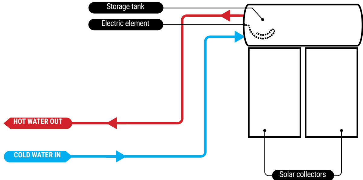
Figure 4. Electric AES system schematic
