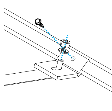
Figure 10. Tank clamp
