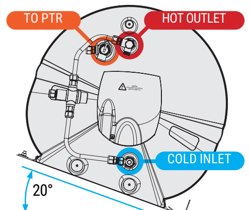
Figure 24. Tank inclination*
