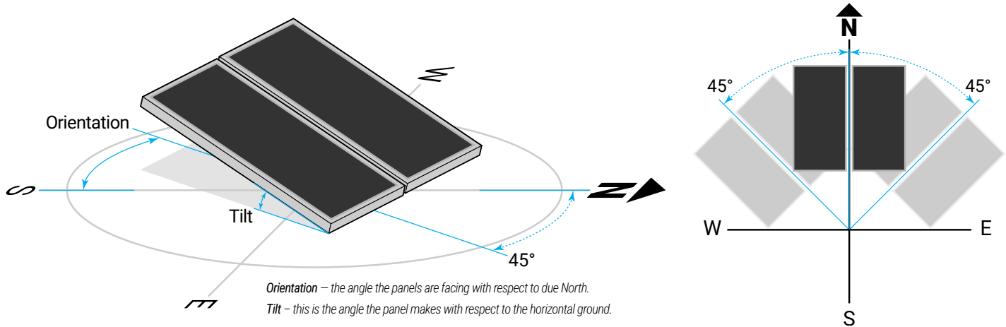
Figure 4. Collector orientation
